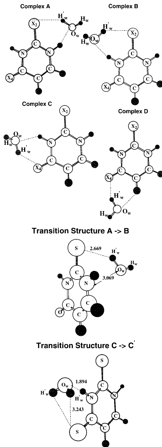
Figure 2. Structures A, B, C, and D of the complexes between the thiouracils and one water molecule. Transition structures in the 2TU–H 2 O and 2,4DTU–H 2 O complexes.
