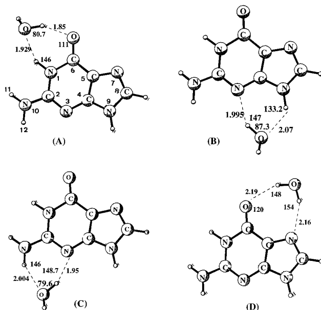
Figure 2. Optimized structures for the A, B, C, and D complexes between guanine and water obtained from B3LYP/6-31+G(d,p) geometry calculations (distances in \text{\AA} , angles in deg).
